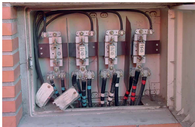
Interior CGP.
